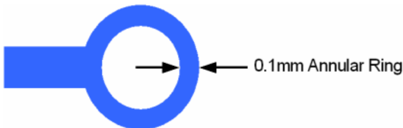
Figure 16 - Annular Ring Illustration
